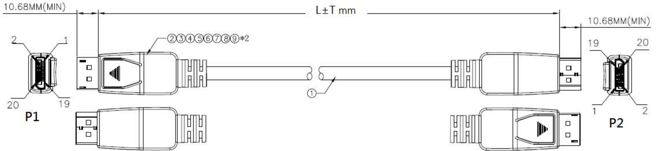
DisplayPort Male
