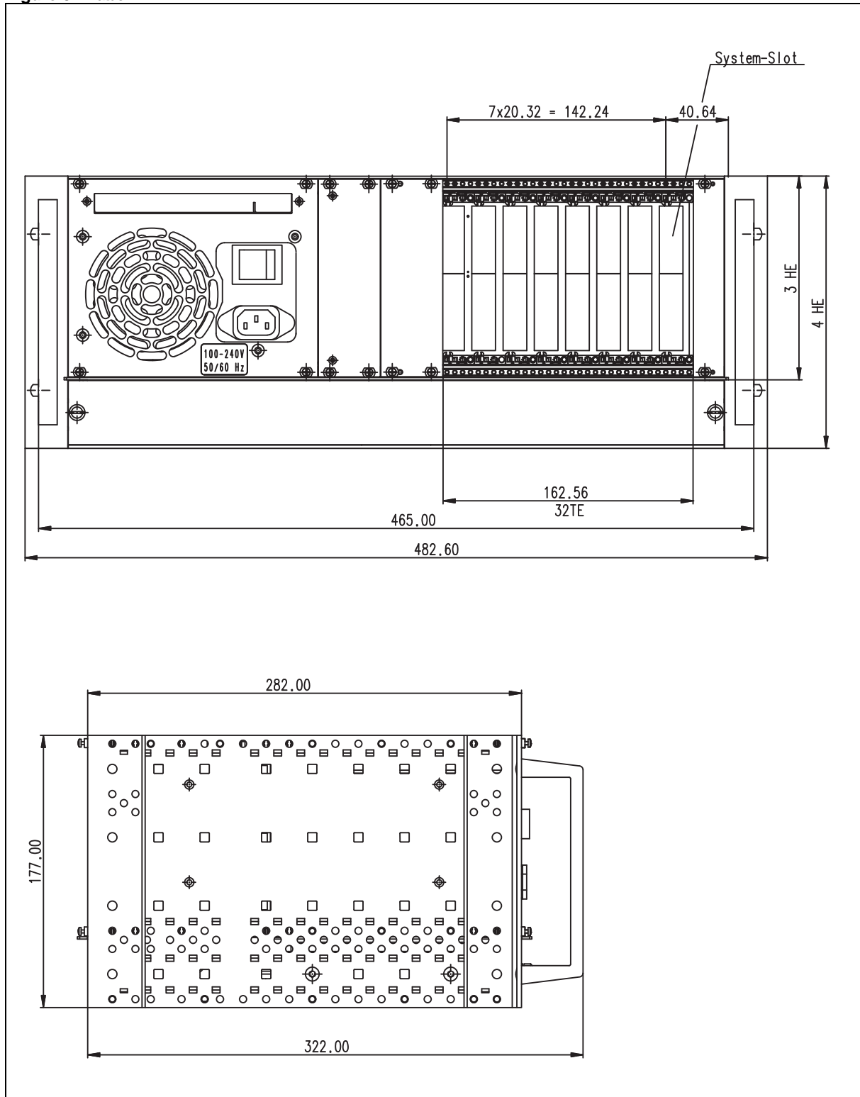
Figure 3: Maße
