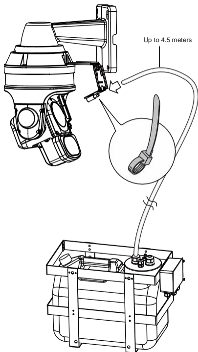
Speed Dome with washer kit.
