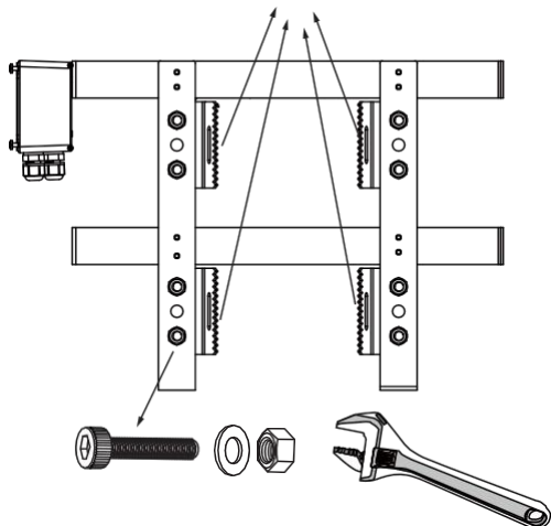
Pole-mount bracket
