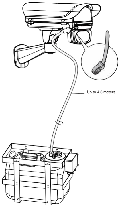
AE housing with washer kit.
