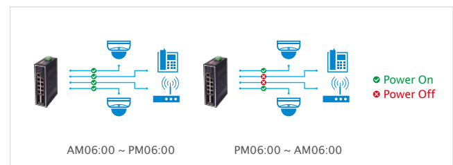
PoE Scheduling
