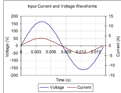
Input AC Current Waveform (ITHD = 5.88%, 50% Load)
